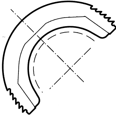
∅52 LINER MEDIUM
