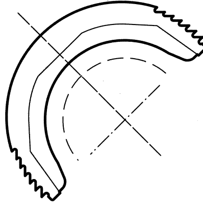
∅54 LINER LARGE
